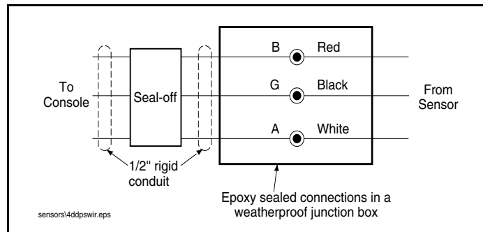
Figure 3. Solid-State Discriminating Dispenser Pan Sensor Wiring Diagram
